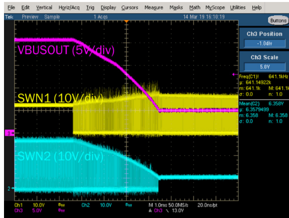
Figure 21. 20 V to 5 V Transition with No Load
