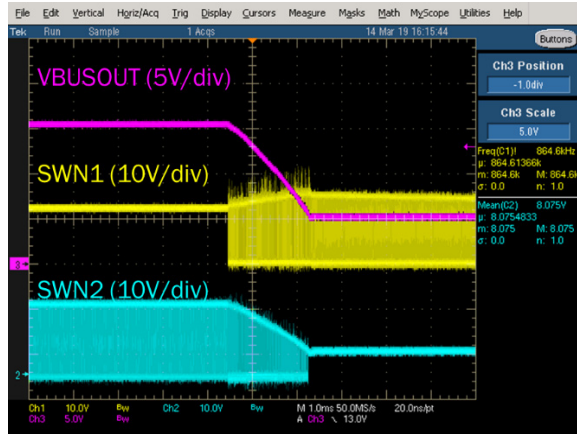
Figure 19. 15 V to 5 V Transition with No Load
