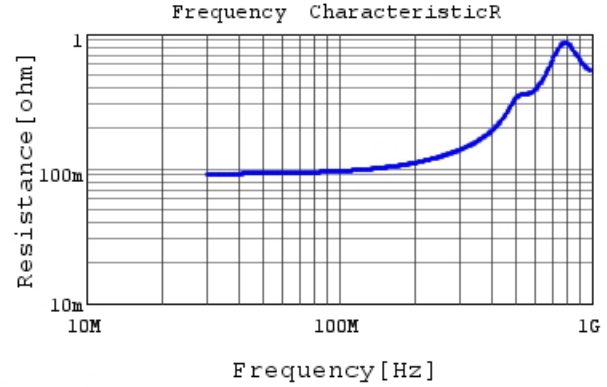
RCE7U2E681J1M1H03A R DC0V, 25degC
