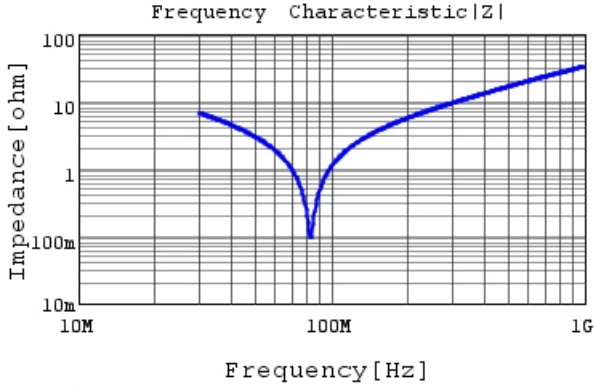
RCE7U2E681J1M1H03A |Z| DC0V, 25degC
