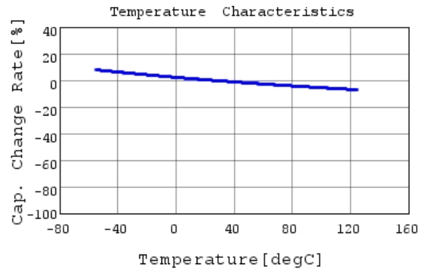
RCE7U2E681J1M1H03A C-Temp. capchange, DC0V,
