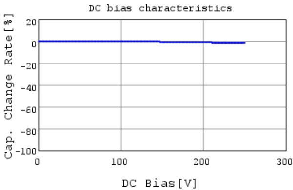
RCE7U2E681J1M1H03A C-DC bias capchange, 25.0
