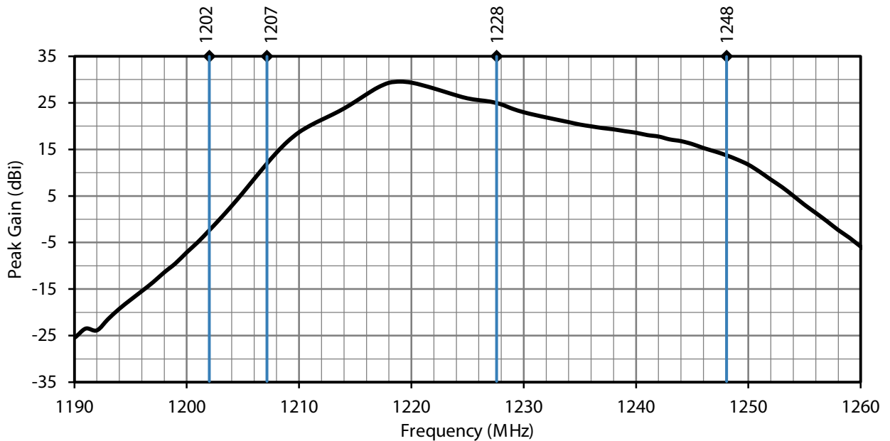
Figure 7. ANT-GNCP-C25L12100 Peak Gain, L2 Band
