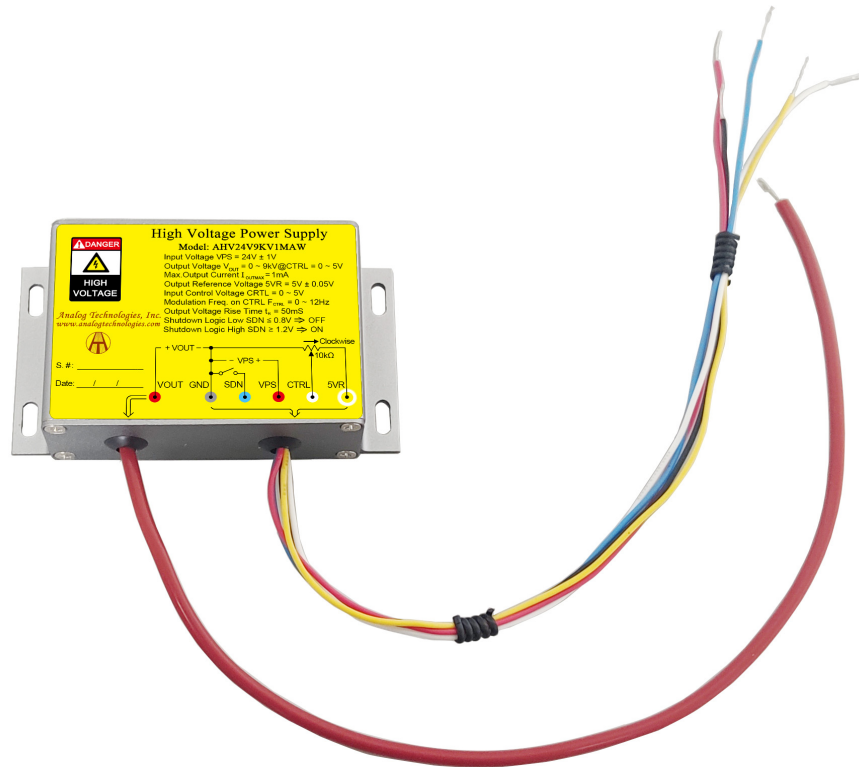
Figure 1.1. Top View of AHV24V9KV1MAW
