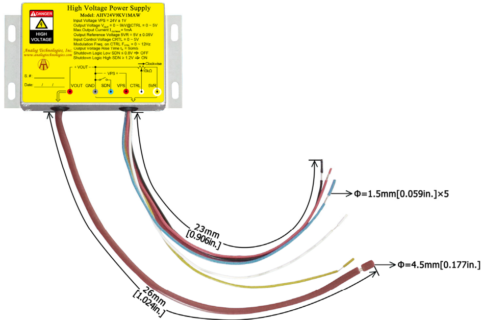
Figure 13. Connecting Lead Wires of AHV24V9KV1MAW
