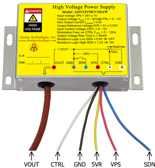
Figure 2. The Connecting Lead Wires of AHV24V9KV1MA
