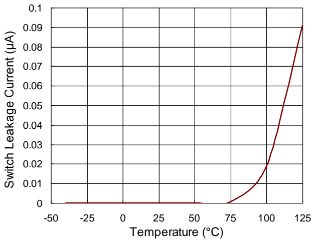
Switch Leakage Current vs. Temperature
