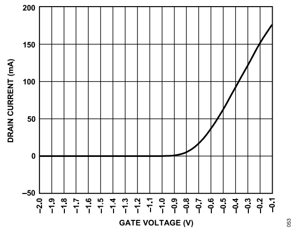
Figure 36. Drain Current vs. Gate Voltage, V_{DD} = 5\text{ V} , I_{DQ} = 85\text{ mA} , V_{GG2} = 1\text{ V}
