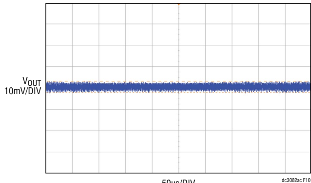
CIRCUIT CONFIGURATION: 16-PHASE SINGLE OUTPUT f_{SW} = 350\text{kHz} , V_{IN} = 12\text{V} , V_{OUT} = 1\text{V} I_{LOAD} = 480\text{A} V_{OUT(P-P)} = 5.3\text{mV} OUTPUT VOLTAGE MEASURED AT V_{OUT} BNC (J11) AC-COUPLING, 20MHz BWL
