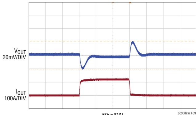
CIRCUIT CONFIGURATION: 16-PHASE SINGLE OUTPUT f_{SW} = 350\text{kHz} , V_{IN} = 12\text{V} , V_{OUT} = 1\text{V} I_{LOAD-STEP} = 0\text{A TO } 120\text{A AT } d_{IL}/d_t = 40\text{A}/\mu\text{s} V_{OUT(P-P)} = 41.9\text{mV} OUTPUT VOLTAGE MEASURED AT V_{OUT} BNC (J11) AC-COUPLING, 20MHz BWL
