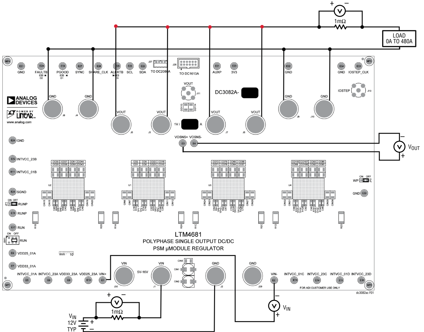
Figure 1. Proper Measurement Equipment Setup for DC3082A-C
