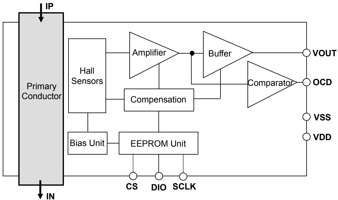
Figure 1. Block diagram of CZ-3813
