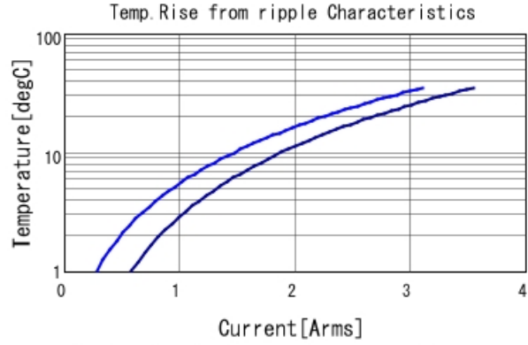
GRT188R70J225KE13 Temp. rise — 500kHz — 1MHz
