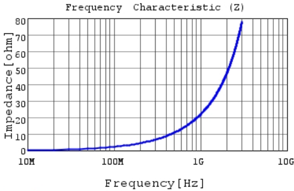
LQG15WH3N5B02 |Z|
