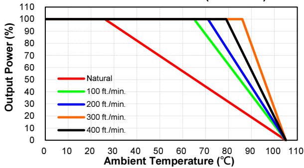
CQB75-300S05 Derating Curve with Heatsink QBT210 (Vin=300V)
