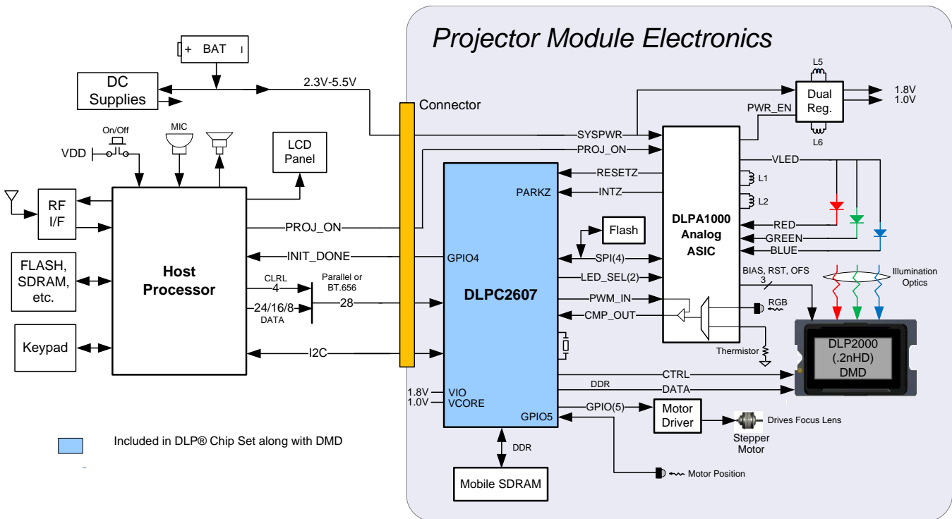
Figure 11. Block Diagram
