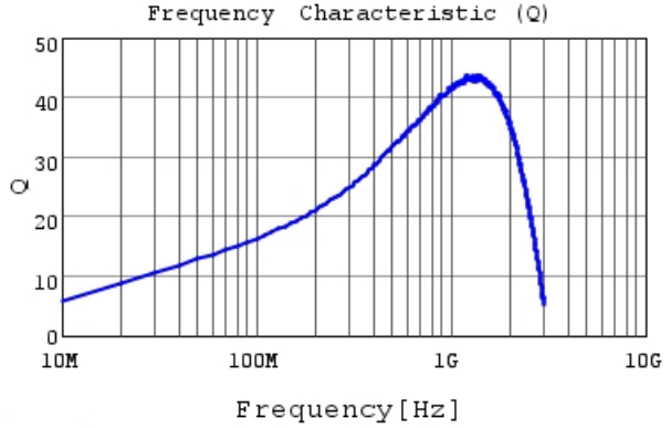
LQG15WZ20NG02 Q
