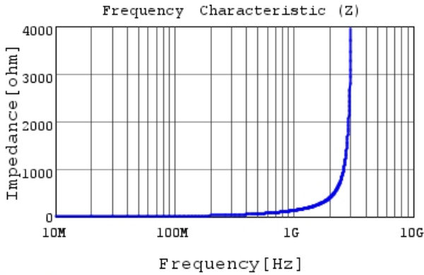
LQG15WZ20NG02 |Z|
