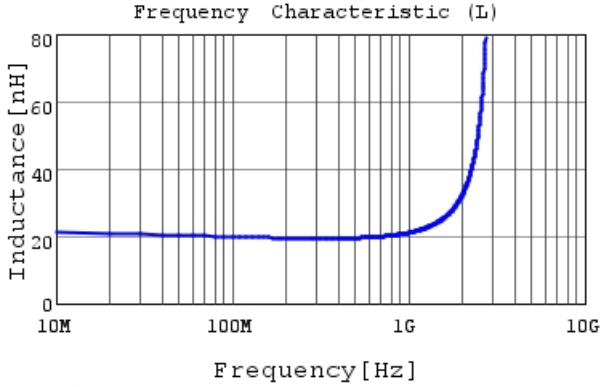
LQG15WZ20NG02 L
