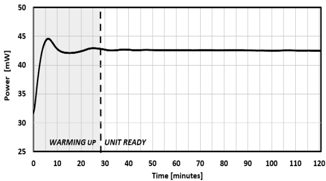
FIG. 15: WARM-UP TIME
