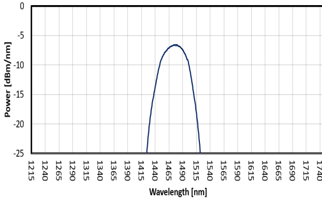
FIG. 5: SLED 4 SPECTRUM
