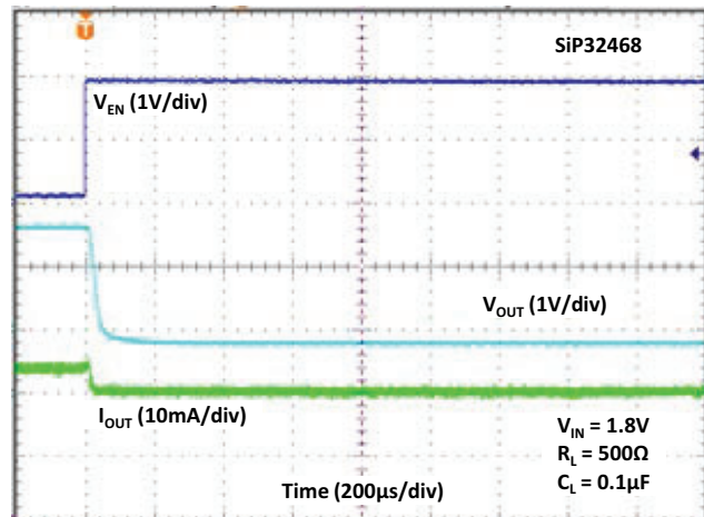
Fig. 33 - Turn-off Time
