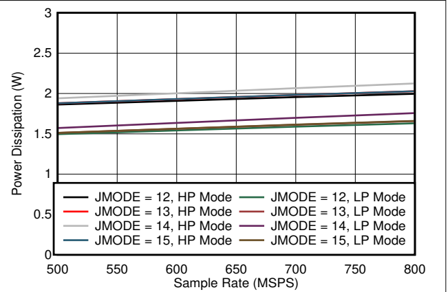
Figure 7-74. Quad Channel, Power Dissipation vs F_S for JMODES 12 - 15
