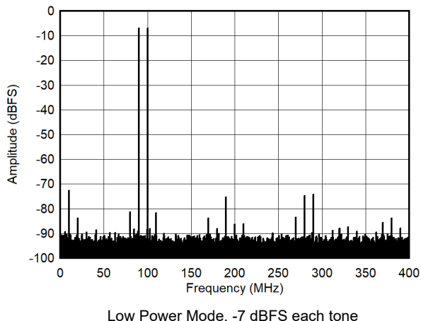
Figure 7-56. Dual Tone FFT at 95 MHz (LP Mode)
