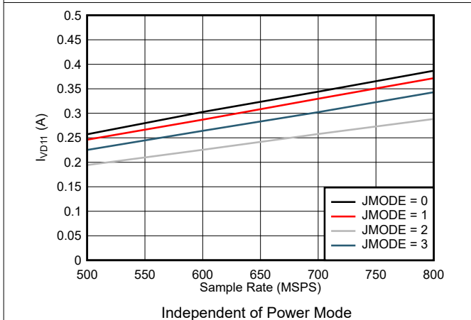
Figure 7-77. Quad Channel, I_{VD11} vs F_S for JMODES 0 - 3
