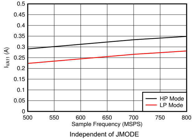
Figure 7-86. Dual Channel, I_{VA11} vs F_S
