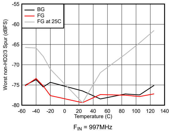
Figure 7-39. Worst non-HD2/3 Spur vs Temperature
