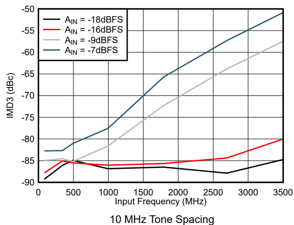
Figure 7-59. IMD3 vs Input Frequency
