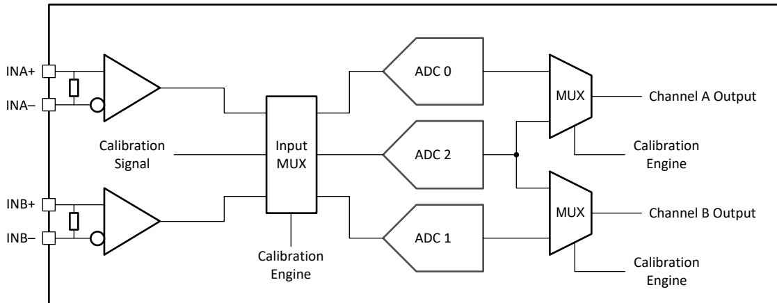
Figure 8-16. DualChannel Calibration System Block Diagram
