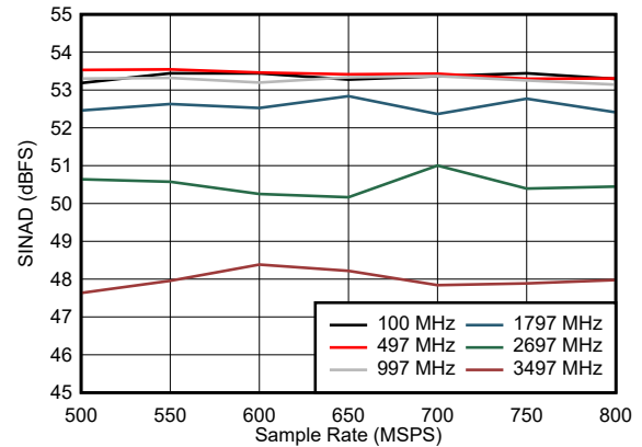
Figure 7-22. SINAD vs Sample Rate
