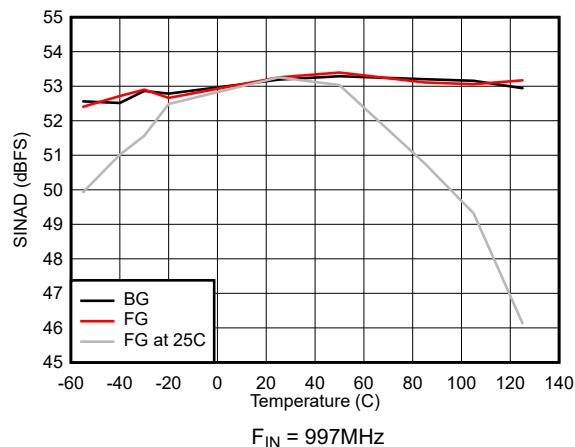
Figure 7-36. SINAD vs Temperature
