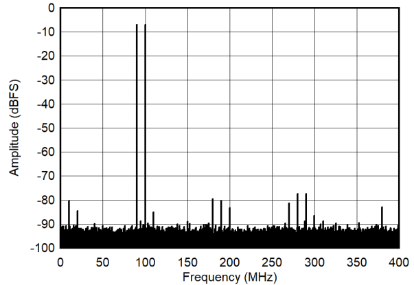
Figure 7-50. Dual Tone FFT at 95 MHz
