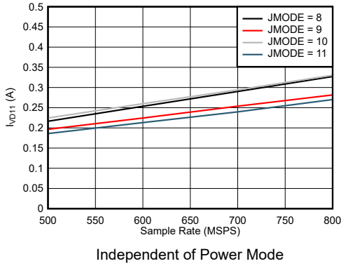
Figure 7-79. Quad Channel, I_{VD11} vs F_S for JMODES 8 - 11
