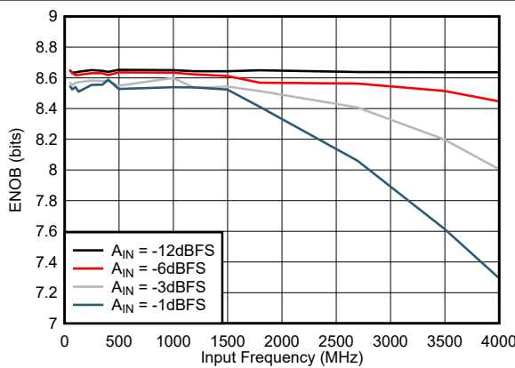
Figure 7-17. ENOB vs Input Frequency
