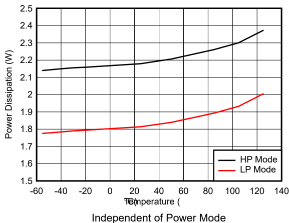
Figure 7-113. Quad Channel, Power Dissipation vs Temperature
