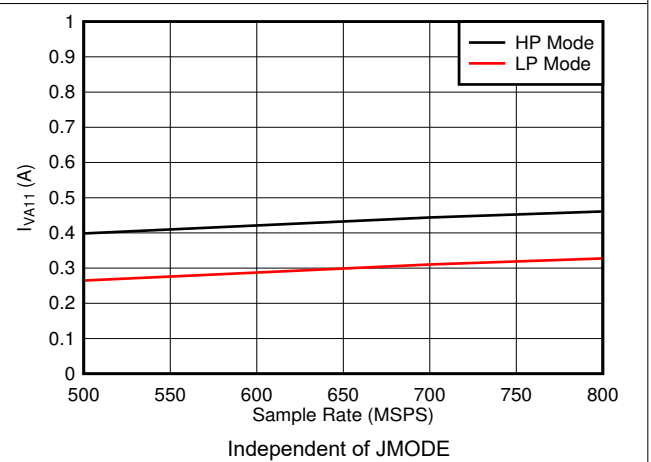
Figure 7-76. Quad Channel, I_{VA11} vs F_S
