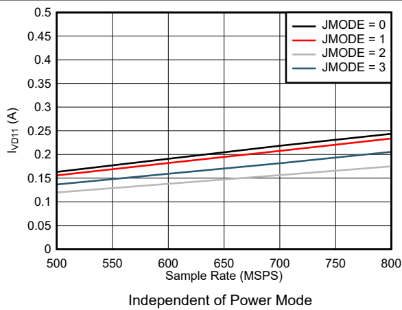
Figure 7-87. Dual Channel, I_{VD11} vs F_S for JMODES 0 - 3
