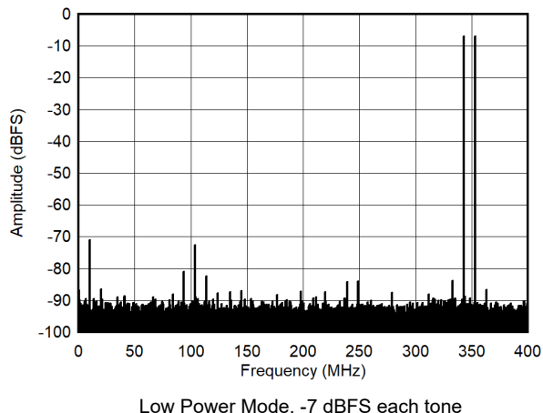
Figure 7-57. Dual Tone FFT at 348 MHz (LP Mode)
