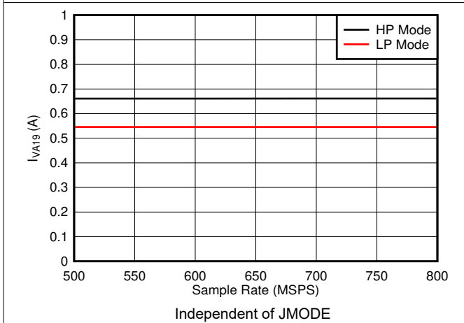
Figure 7-75. Quad Channel, I_{VA19} vs F_S
