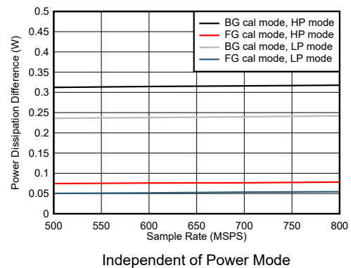
Figure 7-102. Dual Channel, Power Dissipation Change with Calibration Mode
