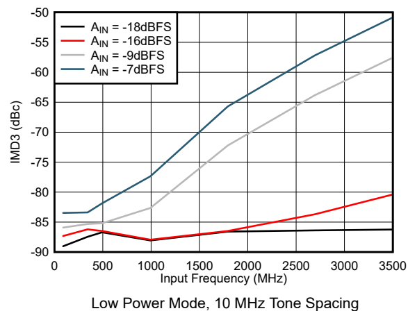
Figure 7-60. IMD3 vs Input Frequency (LP Mode)
