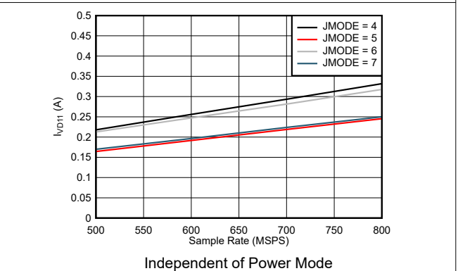
Figure 7-78. Quad Channel, I_{VD11} vs F_S for JMODES 4 - 7
