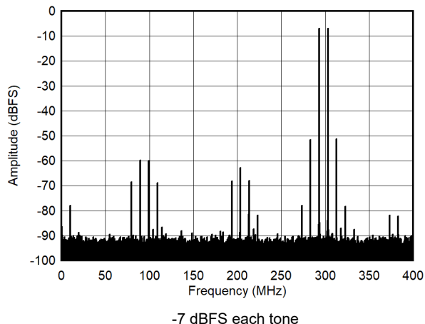
Figure 7-55. Dual Tone FFT at 2698 MHz
