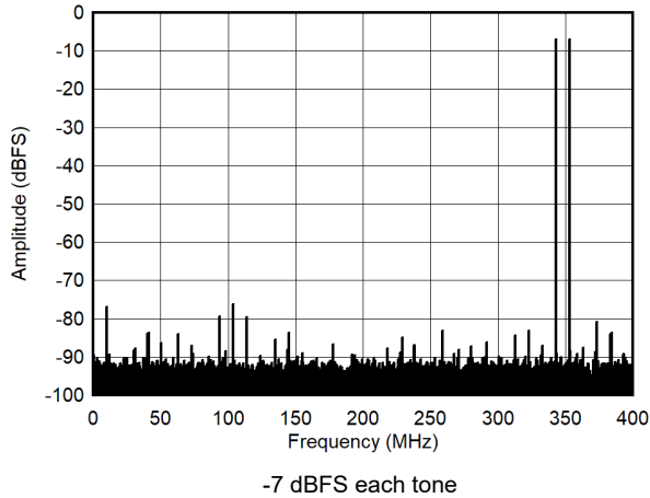
Figure 7-51. Dual Tone FFT at 348 MHz
