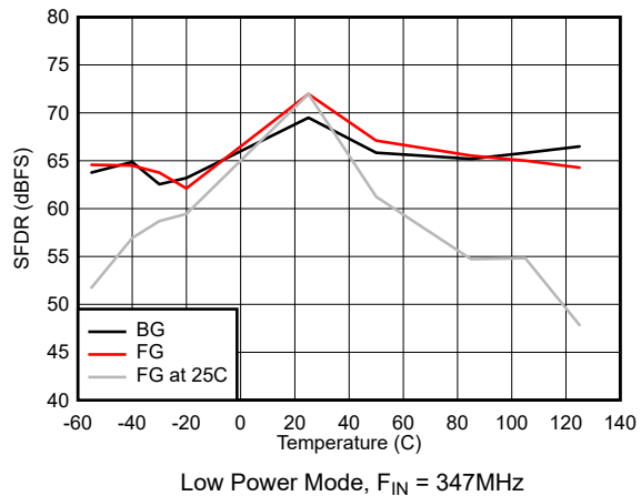
Figure 7-41. SFDR vs Temperature
