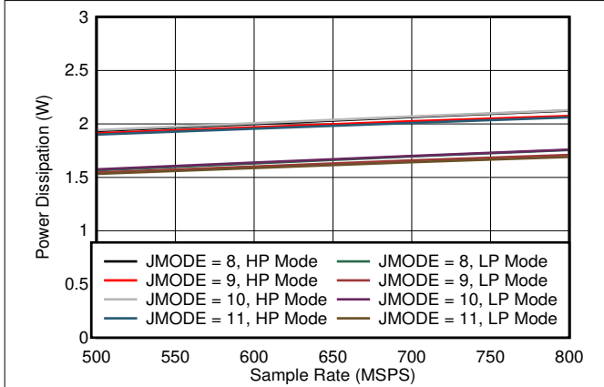
Figure 7-73. Quad Channel, Power Dissipation vs F_S for JMODES 8 - 11
