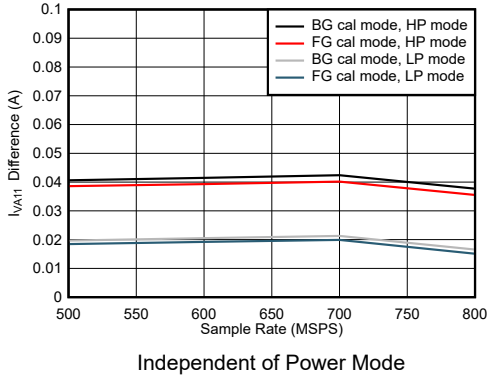
Figure 7-109. Single Channel, I_{VA11} Change with Calibration Mode
