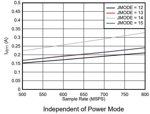
Figure 7-80. Quad Channel, I_{VD11} vs F_S for JMODES 12 - 15
