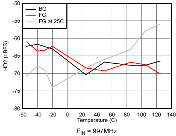
Figure 7-37. HD2 vs Temperature
