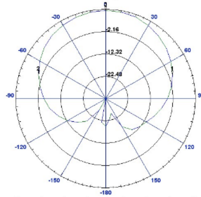
Vertical plane pattern V
