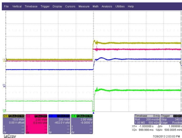
Figure 31. PS-ON, [200 ms/div]
