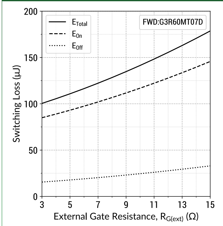
Figure 23: Inductive Switching Energy v/s R_{G(ext)} ( V_{DD} = 450V )
