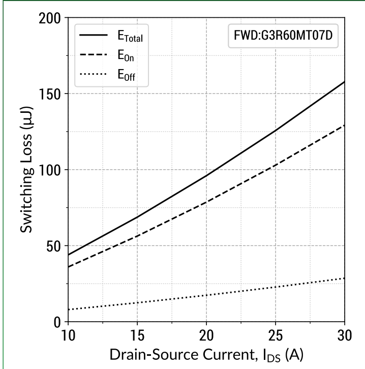
Figure 21: Inductive Switching Energy v/s Drain Current ( V_{DD} = 350V )
