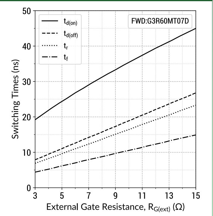
Figure 24: Switching Time v/s R_{G(ext)} ( V_{DD} = 450V )
