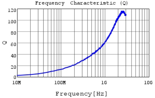
LQG15WZ1N7B02 Q
