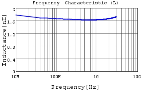
LQG15WZ1N7B02 L
