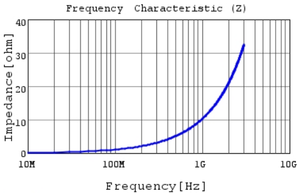
LQG15WZ1N7B02 |Z|
