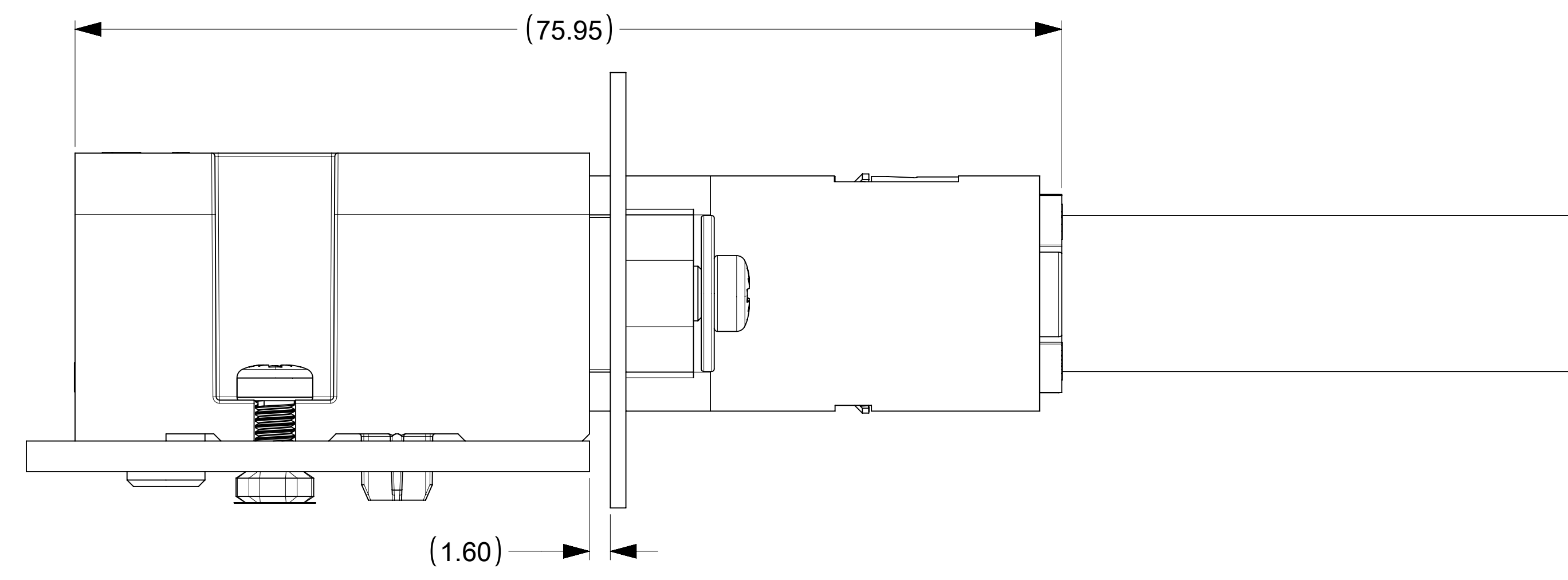
ASSEMBLED AND MATED WITH RA HEADER_SOLDER TAIL VERSION (2155106241)
