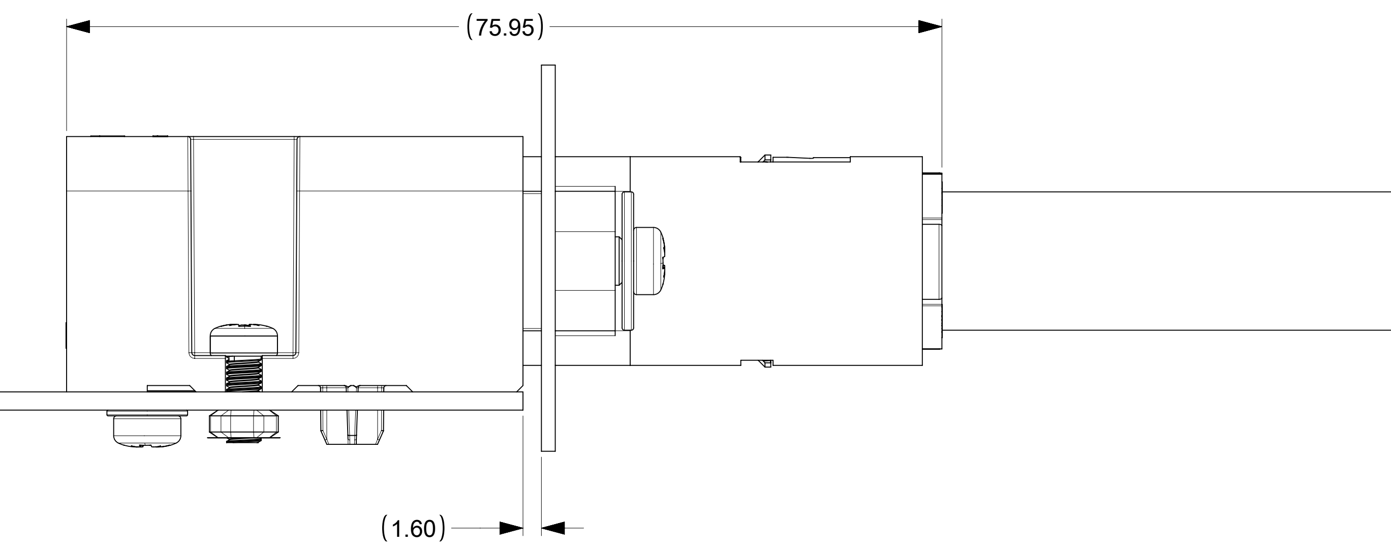
ASSEMBLED AND MATED WITH RA HEADER_SCREW MOUNT VERSION (2155106031)
