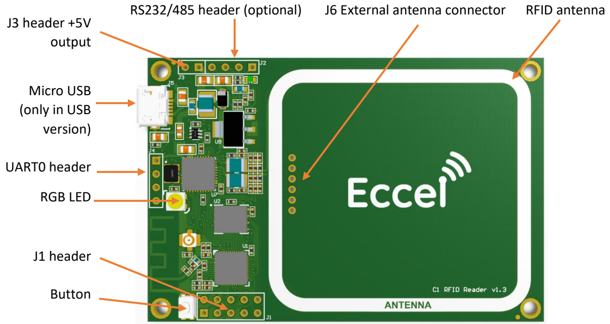
Figure 1. Pepper C1 (USB version)
