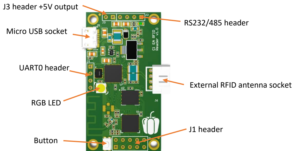
Figure 2. Pepper C1 EA (external antenna)
