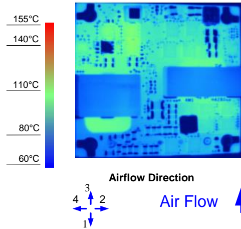
Figure 8. Thermal Image for Airflow Direction 3 (11A output, 55°C ambient, 200 LFM, typical Vin, open frame, unit soldered onto a fixture board)
