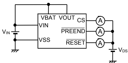
Figure 7 Test Circuit 3
