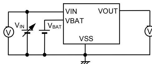
Figure 8 Test Circuit 4
