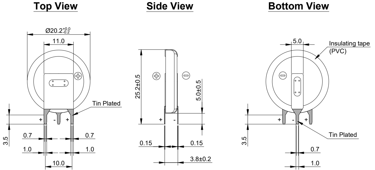
Figure 7. SCR2032VC02S/1225 Mechanical Layout
