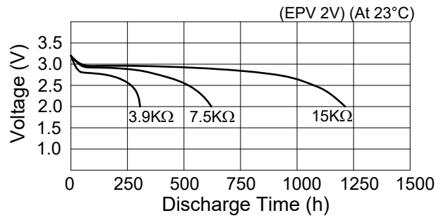
Figure 1. Discharge Characteristics
