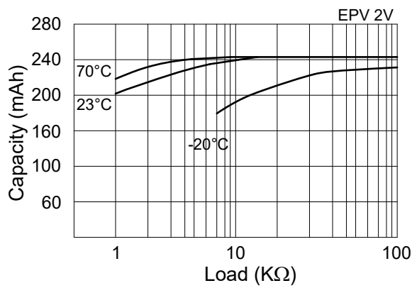
Figure 5. Load-Capacity
