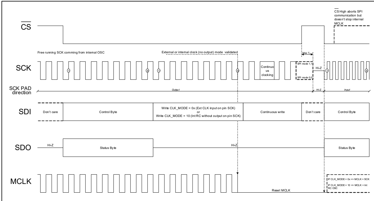
FIGURE 6-16: MCP3565R Transition from CLK\_SEL[1:0] = 11 to 0x/10 .
