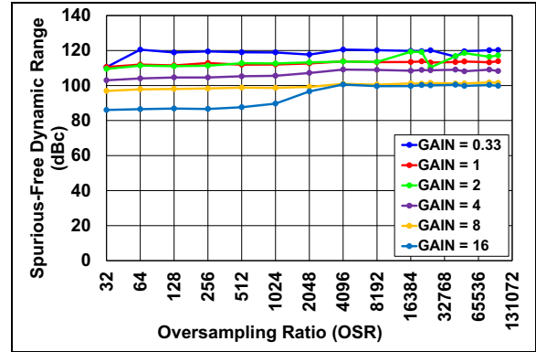
FIGURE 2-17: SFDR vs. OSR Internal V_{REF} .
