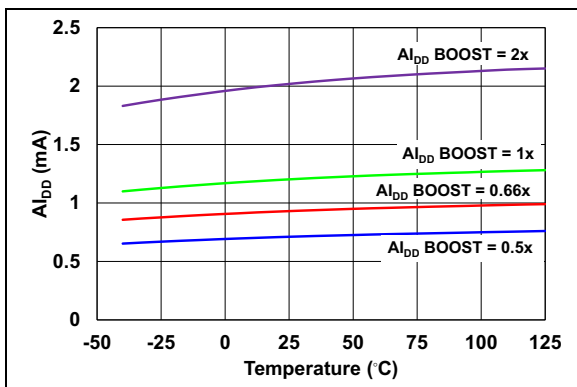
FIGURE 2-57: DI_{DD} and Al_{DD} vs. Temperature.
