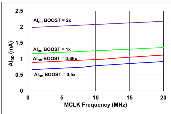
FIGURE 2-56: Al_{DD} vs. MCLK (Internal V_{REF} ).
