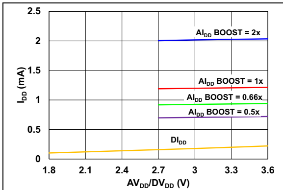
FIGURE 2-55: DI_{DD} and Al_{DD} vs. DV_{DD} and AV_{DD} .
