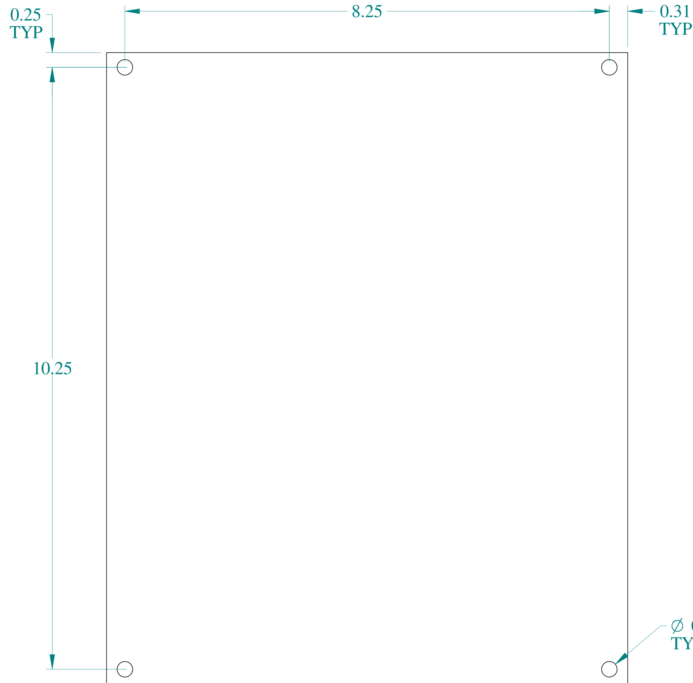
FRONT VIEW
