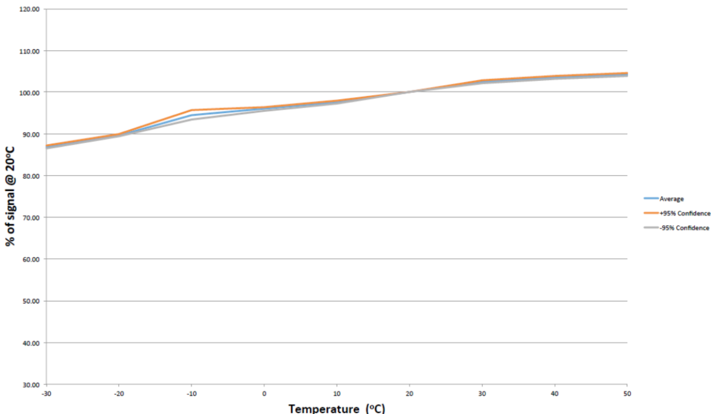
Output Temperature Coefficient Data
