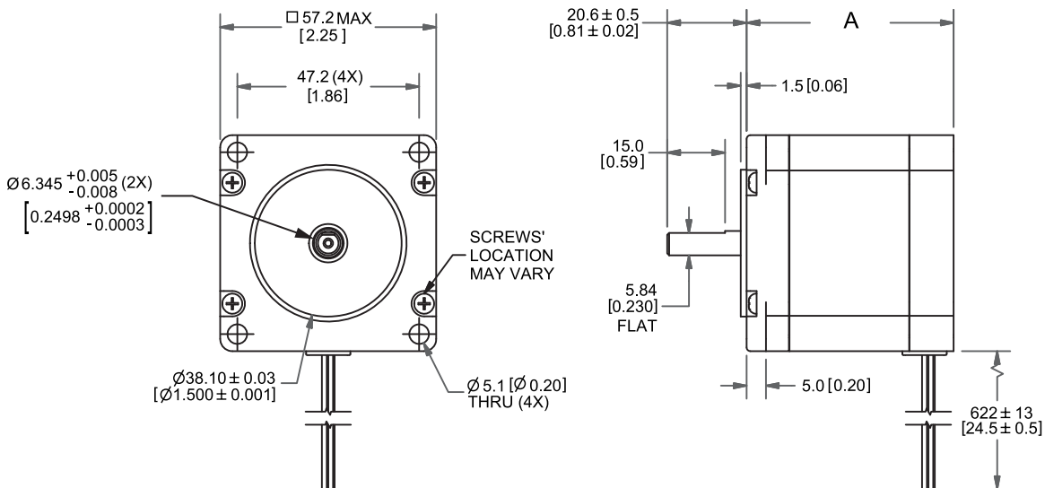
5718X-01S 24VDC, 1.4 Amps/Phase, Bipolar Series, 1/2 Stepping 5718X-01P 24VDC, 2.8 Amps/Phase, Bipolar Parallel, 1/2 Stepping
