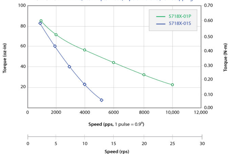
5718X-01S 24VDC, 1.4 Amps/Phase, Bipolar Series, 1/2 Stepping 5718X-01P 24VDC, 2.8 Amps/Phase, Bipolar Parallel, 1/2 Stepping
