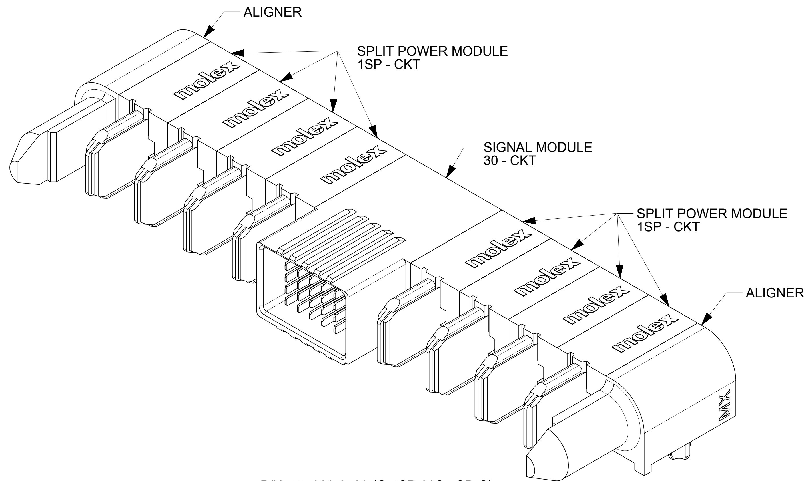
P/N: 171088-8429 (G-4SP-30S-4SP-G)
