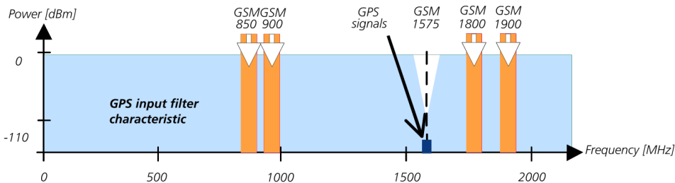
Figure 37: Out-band jamming signals
