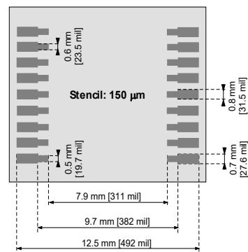
Figure 10: MAX-7 paste mask
