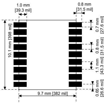
Figure 8: MAX-7 footprint
