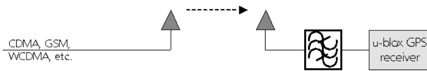
Figure 38: Measures against in-band jamming
